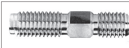
Figure 5. Catalog Number STUD-T The Copper Alloy Stud with its extended length allows for threading into the connector prior to mating the bushing and terminator interfaces. Blunt start threads on the stud help eliminate cross-threading. Stud threads into an industry standard 600 A bushing.
