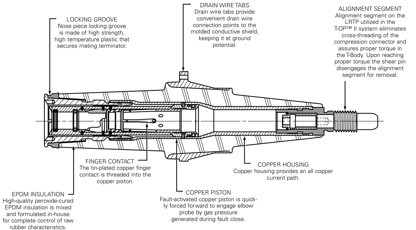
Figure 1. Loadbreak Reducing Tap Plug with 200 A and 600 A interfaces. Field proven, all copper alloy current path ensures the coolest operating temperatures and best reliability.
