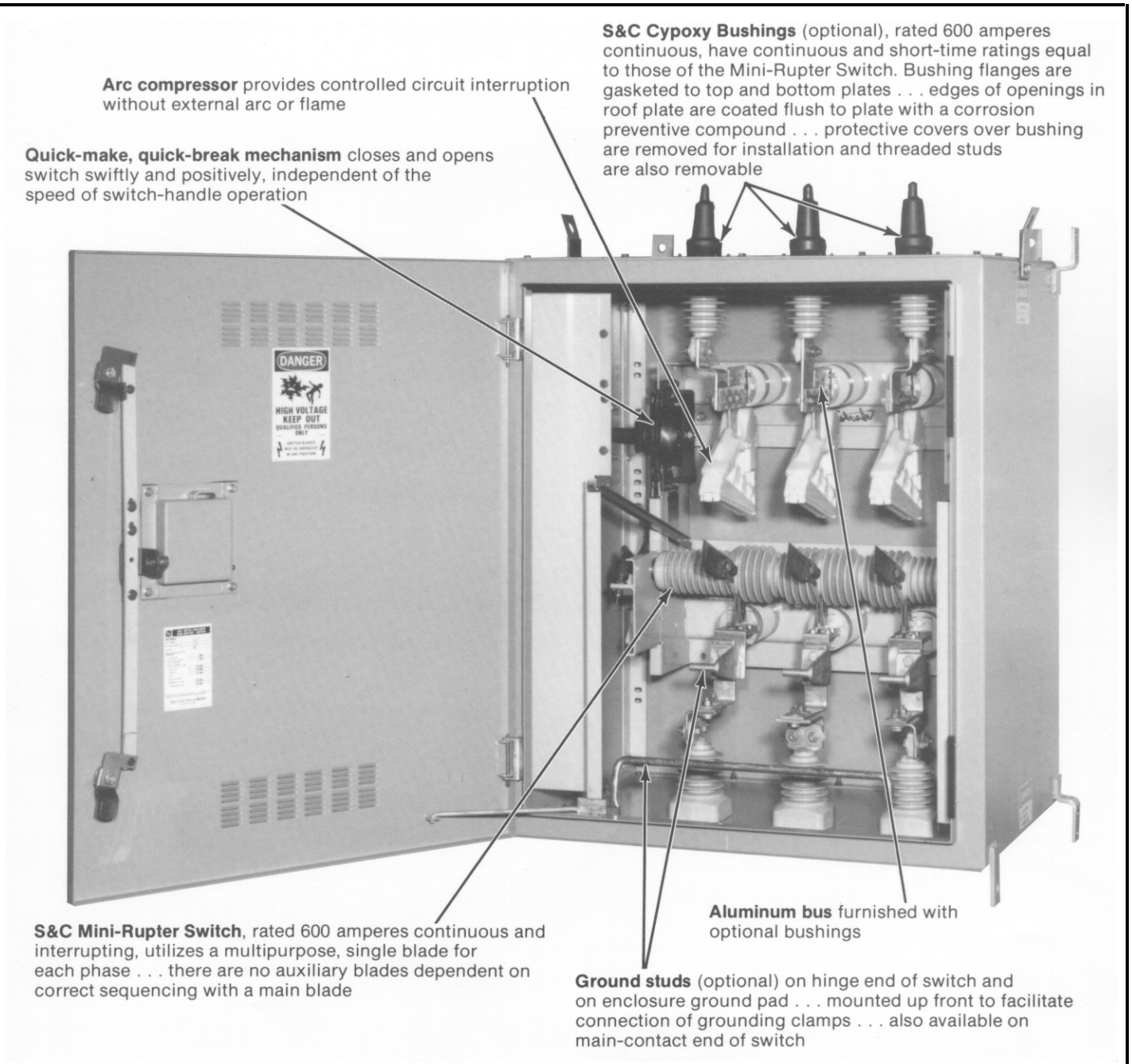
Interior view of metal-enclosed switch with the optional dual-purpose front barrier completely removed.
